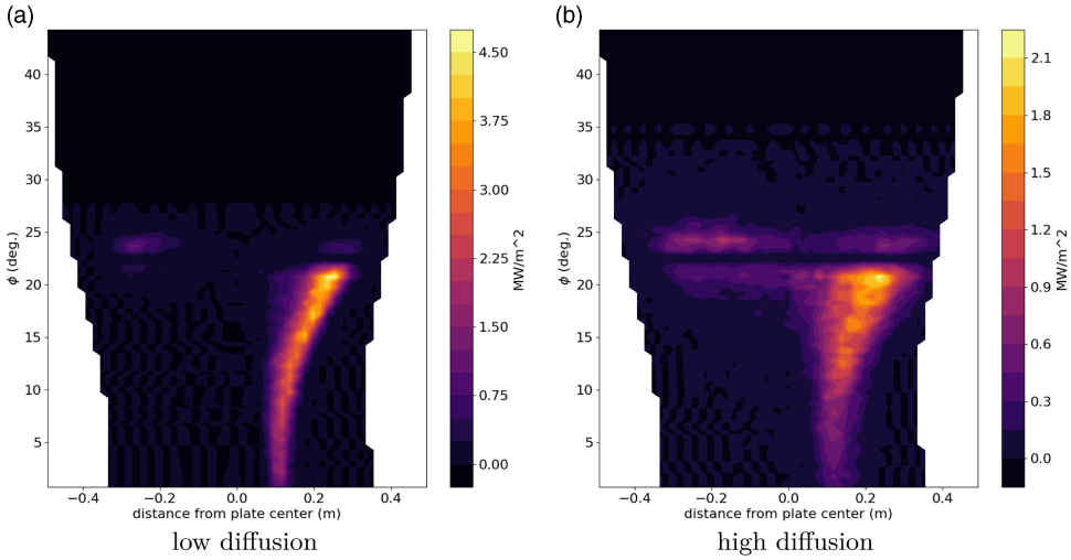
FIGURE 11. Heat flux from EMC3-Lite for classical divertor with total power entering SOL is P_{\text{SOL}} = 8 \text{ MW} , electron temperature T_{e,\text{sep}} = 100 \text{ eV} and electron density n_{e,\text{sep}} = 1 \times 10^{20} \text{ m}^{-3} at separatrix. Thermal diffusion coefficient (a) \chi = 0.1 \text{ m}^2\text{s}^{-1} , (b) \chi = 1.0 \text{ m}^2\text{s}^{-1} .
