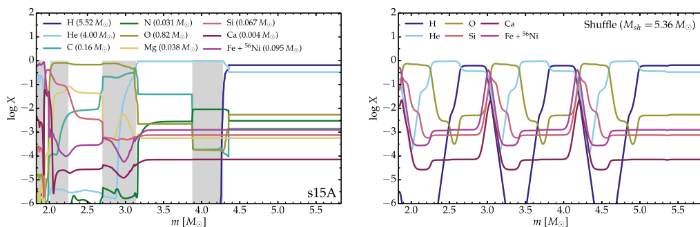
Figure 6. An illustration of the treatment of macroscopic mixing in 1D. On the left we see the chemical composition of the original SN model (based on the S15A ejecta model of Woosley & Heger (2007)) – the onion-like chemical structure of the ejecta is clearly evident. On the right the distinct chemical zones have been broken into three fragments, and these have then been shifted in radius. See Dessart & Hillier (2020b) for further details. Reproduced from: “Radiative-transfer modeling of supernovae in the nebular-phase. A novel treatment of chemical mixing in spherical symmetry” (figure 1), Dessart & Hillier (2020b).
