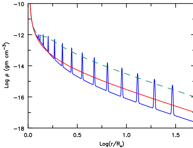
Figure 2. An illustration of the density distribution in three models for AzV83 – all models have the same average mass-loss rate. The red solid curve is for a smooth density distribution and the blue solid curve is for the shell model with an average wind VFF of 0.1. The green dashed curve illustrates the clump density in the VFF model (but recall that the interclump medium is void) with VFF = 0.1. By adjusting model parameters it is possible to vary the number of clumps, clump size and the density of the interclump medium. Reproduced from: “Using Shell models to investigate clumping in the wind of the O7Iaf+ supergiant AzV83” (figure 3), Flores & Hillier (2021).
