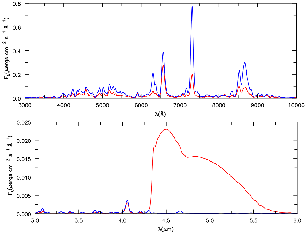
Figure 7. Spectra for a model of a supernova similar to SN 1987A. The model has classical mixing (i.e., not the shell approach). The blue line shows the spectrum at an age of 330 days without cooling, while the (preliminary) model shown in red has CO cooling. CO cooling, primarily by the fundamental band, weakens optical features such as O I \lambda\lambda 6300, 6364, Ca II \lambda\lambda 7291, 7233, and Ca II \lambda\lambda 8498, 8542, 8662. Longward of 4.3\,\mu\text{m} we see the strong emission by the fundamental band of CO which completely dominates this spectral region.
