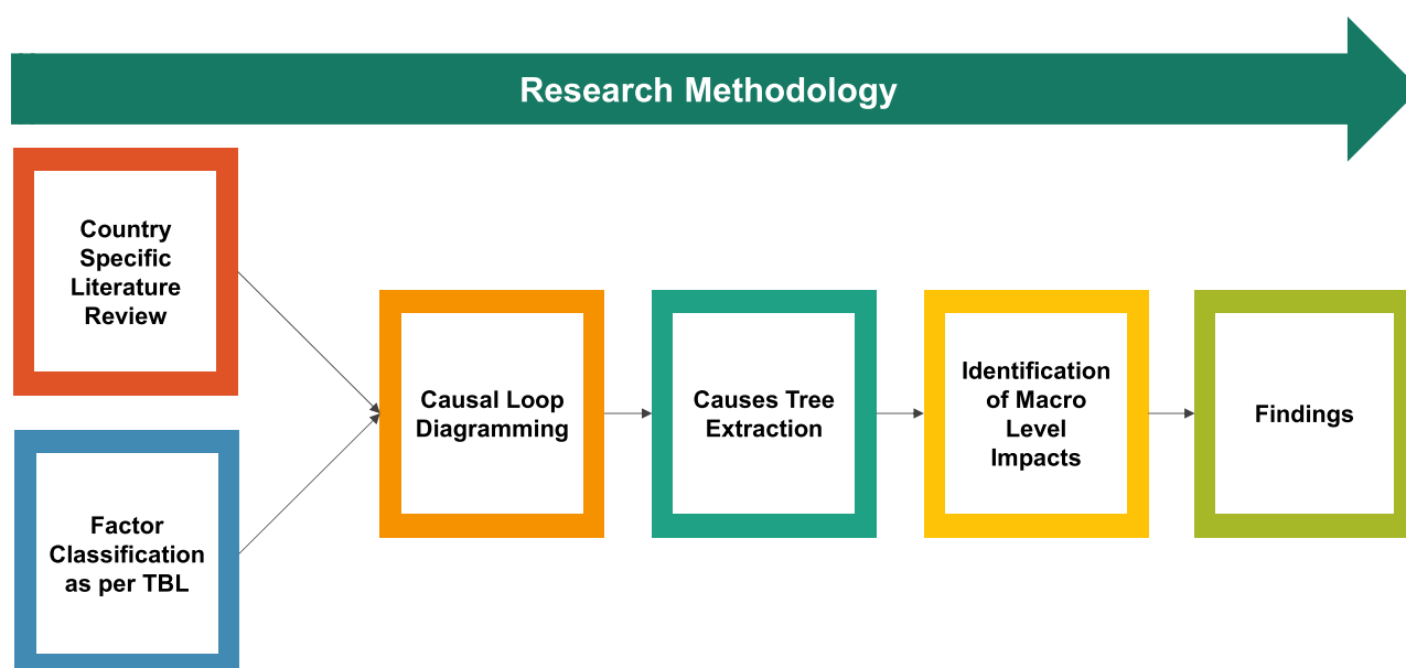
Figure 2. Study methodology.
