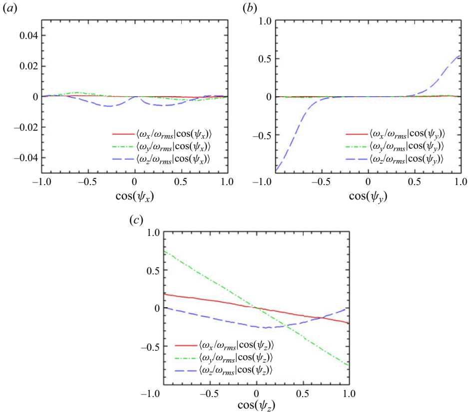
Figure 10. Average of normalized vorticity components \omega_i / \omega_{rms} conditioned on the cosine of interface orientation \cos(\psi_j) at M_c = 1.8 and at \tau = 1750 .
