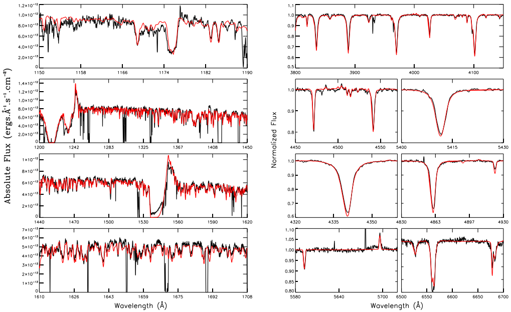
Figure 7. Preliminary CMFGEN fits (red/grey) to UV (HST/STIS/E140M from ULLYSES, left) and optical (VLT/Xshooter from XShooterU, right) spectroscopy (black) of the LMC star Sk-68° 16 (O7 III), courtesy of JC Bouret.
