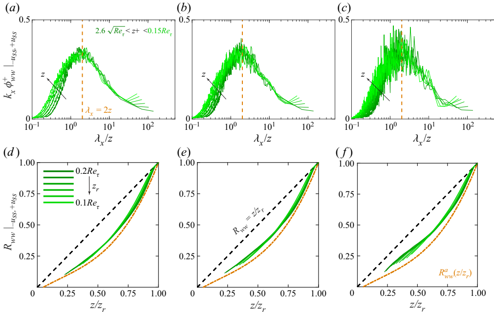
Figure 15. (a–c) Conditionally averaged premultiplied 1-D spectra of w -fluctuations plotted \overline{vs} \lambda_x/z at various z^+ within the log region. (d–f) Correlation between w -fluctuations at z and z_r , normalized by \overline{w^2}(z_r) for various z_r . Here, both the spectra and the cross-correlations are computed from the extracted w -flow fields associated with -u_{ss} and +u_{ss} detected in the LFOV PIV data at Re_\tau \approx 7500 , for varying thresholds of the streamwise lengths associated with the superstructures: (a,d) L_x \gtrsim 3\delta , (b,e) L_x \gtrsim 3.8\delta and (c,f) L_x \gtrsim 4.5\delta . In (a–c), the dashed golden line represents the linear scaling, \lambda_x = 2z . In (d–f), the dashed black line corresponds to the linear relationship, z/z_r while the dash-dotted golden line corresponds to R_{ww}^a defined in (3.2).
