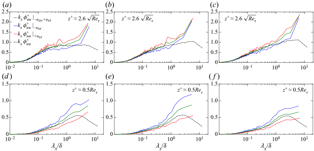
Figure 7. (a–f) Premultiplied 1-D spectra of the u -fluctuations plotted vs \lambda_x/\delta at (a–c) z^+ \approx 2.6\sqrt{Re_\tau} and (d–f) z^+ \approx 0.5Re_\tau for LFOV PIV data at Re_\tau \approx (a, d) 2500, (b, e) 5000 and (c, f) 7500. Dashed black lines correspond to the mean spectra obtained by ensembling across 3000 PIV images of the full flow field. While, the solid blue and red lines represent conditional spectra computed from the u -flow field extracted based on identification of a -u_{ss} and +u_{ss} , respectively. The spectrum in green is computed by ensembling across both -u_{ss} and +u_{ss} .
