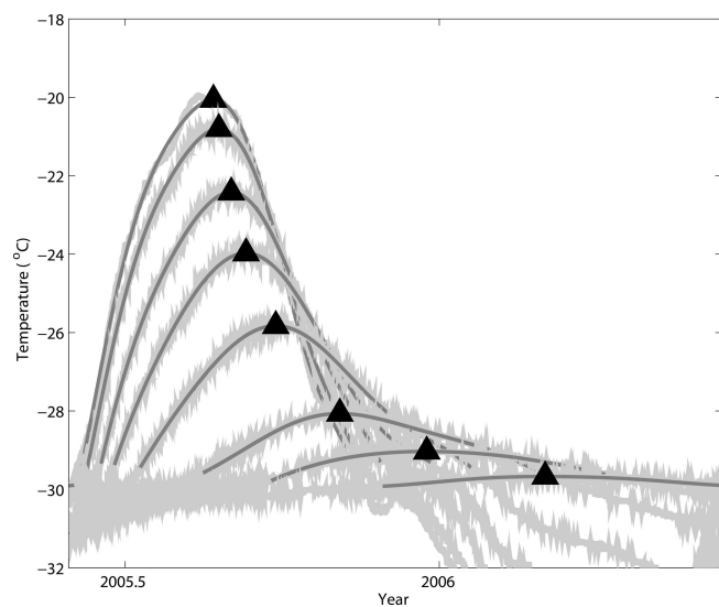
Fig. 3. Annual temperature maxima (triangles) identified by third-order Fourier series fits (dark curves) to data (light curves).
