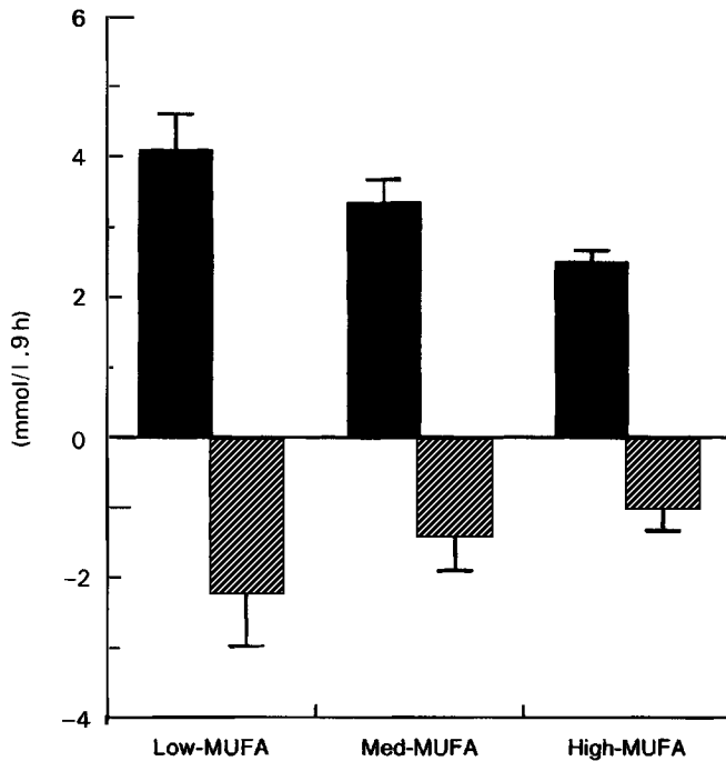
Fig. 2. Areas under the postprandial response curve (■) and incremental areas under the postprandial response curve (▨) for non-esterified fatty acids in subjects consuming low-, medium- and high-monounsaturated fatty acid (MUFA) meals. Values are means for fifteen subjects with their standard errors represented by vertical bars. For details of meals see p. 539 and Table 1.
