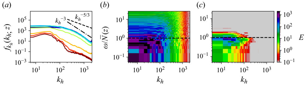
Figure 6. (a) Horizontal wavenumber spectrum f_{k_h}(k_h, z) at a range of heights in simulation HR, compared with an isotropic and axisymmetric turbulence scaling k_h^{-5/3} , k_h^{-3} , shown as dashed and dot-dashed black lines, respectively. Line colours as in figure 5. (b,c) Energy spectrum E at (z-H)/z_{max} = 0.25, 1.4 . The black dashed line indicates \omega/\bar{N}(z) = 1 .
