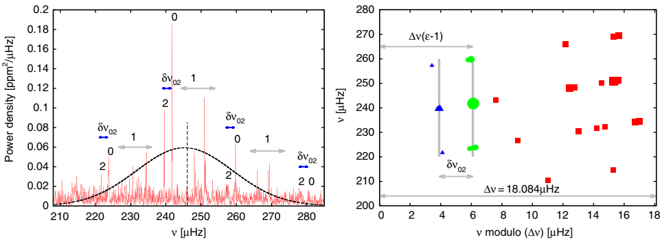
Figure 1. Left: the power density spectrum of KIC 5110739 indicating oscillations. The black dashed curve shows a heavily smoothed power spectrum indicating the power excess envelope of the solar-like oscillations. The black dashed vertical line represents \nu_{\max} = 246.08 \nu\text{Hz} . The numbers indicate the degree, l , of the modes and \delta\nu_{02} represent the small frequency separation ( \sim 2.4 \nu\text{Hz} ). Right: Echelle diagram of KIC 5110739 showing the frequencies (red squares, green points and blue triangles) as determined from the power spectrum: modes with l=0 , l=1 , and l=2 are represented with circles, squares and triangles, respectively.
