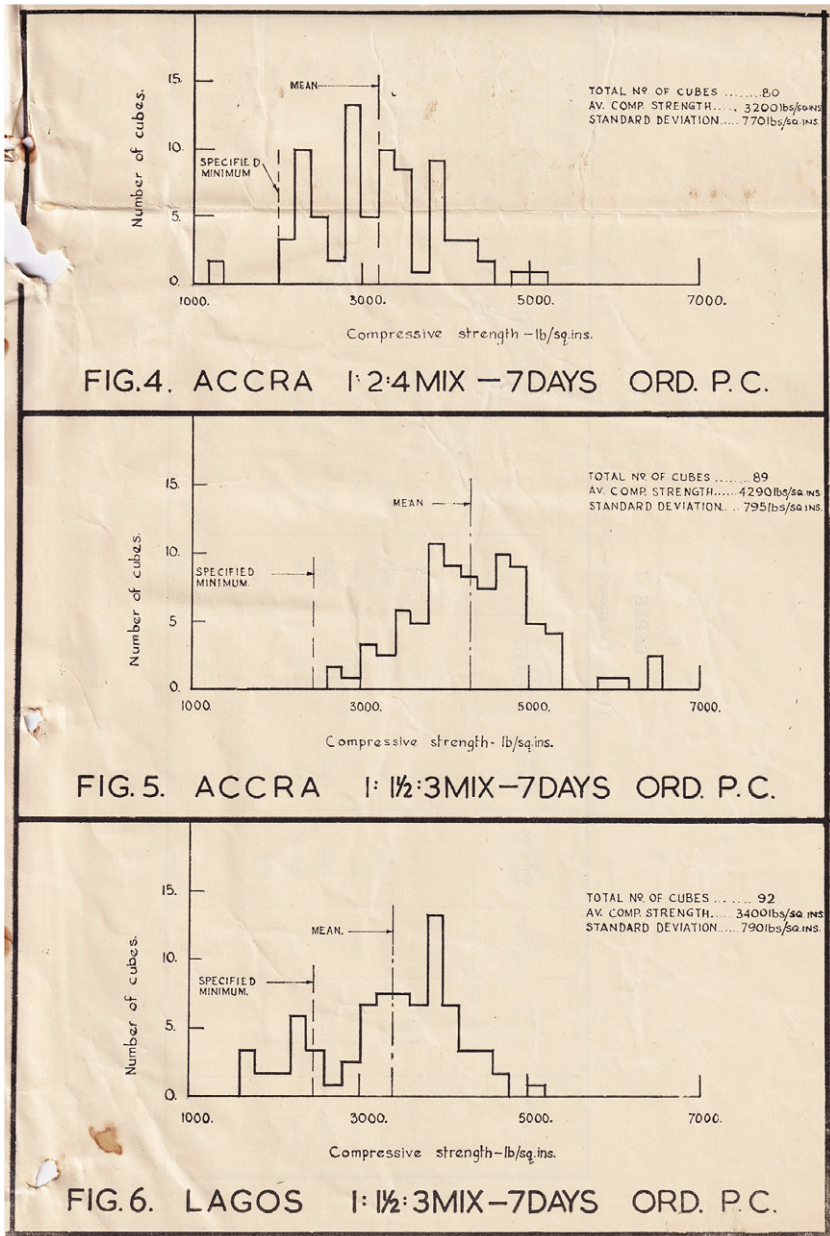
Figure 3. Compressive strength of concrete cubes. "Quality of Concrete," West African Building Research Institute Information Sheet 4, August 1954.
