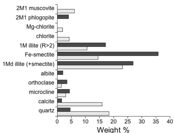
Fig. 2 Summary of the mineralogy of two French green clays used to treat Buruli ulcer in the Ivory coast (Argicur = dark bars; Argiletz = light bars) (reproduced, with permission, from Williams, 2017)
