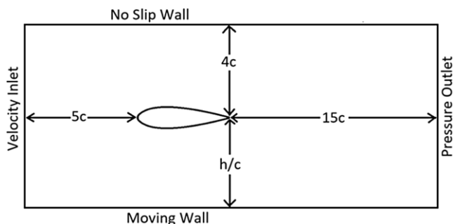
Figure 2. Aerofoil domain size and boundary conditions.
