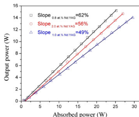
Figure 8. Laser performance of the Nd:YAG ceramic lasers.
