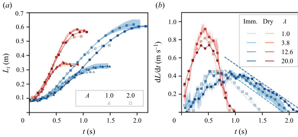
Figure 5. (a) Front position evolution L(t) for dry (red) and immersed (blue) columns, and for A \simeq 1 ( \triangle ) and A \simeq 2 ( \square ). (b) Front velocity evolution dL/dt for dry and immersed columns with aspect ratio A \simeq 2 . Shaded areas represent the variability between repetitions, with envelopes indicating the minimum and maximum values, and markers and continuous lines are the average of them. In (b), the dashed lines represent the collapse acceleration magnitudes d^2L/dt^2 for immersed columns during the collapse deceleration phase.
