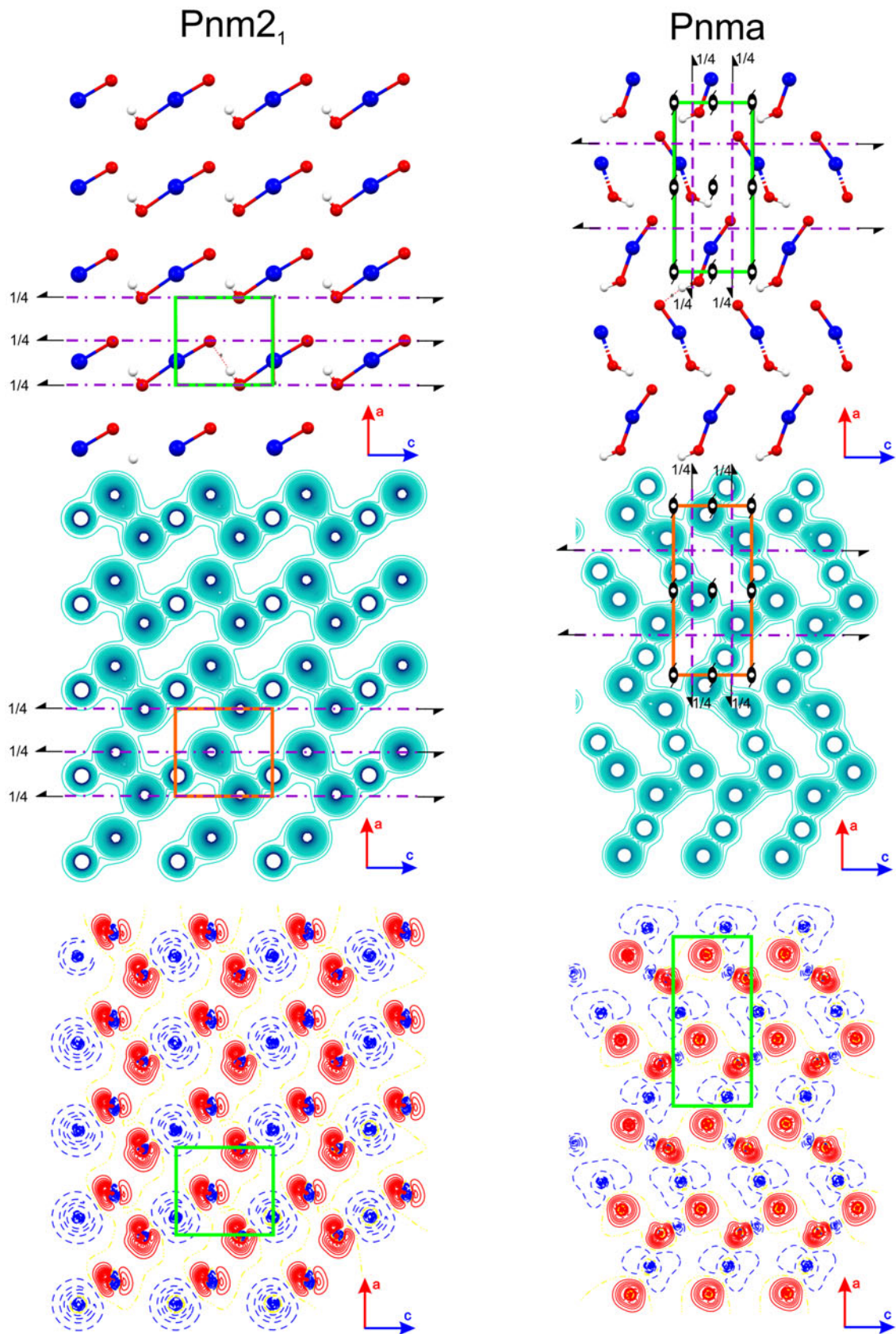
Figure 7. Comparison of the atomic arrangements in the \alpha -AIOOH and \delta -AIOOH phases. The 1st row: atomic positions and symmetry elements with unit cells defined. The 2nd row: unit cell with symmetry elements with the total charge-density distributions in the background. The 3rd row: deformation electron density distributions – views along the y-axis.
