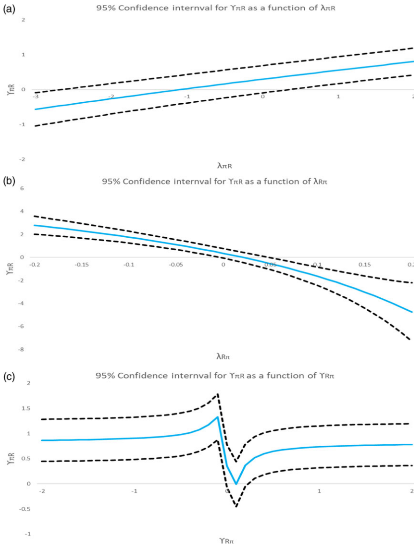
Figure 3. The long-run impact of the interest rate on inflation in UK. Note: annual data 1310–2018; the dashed lines represent the two-standard error bands.
