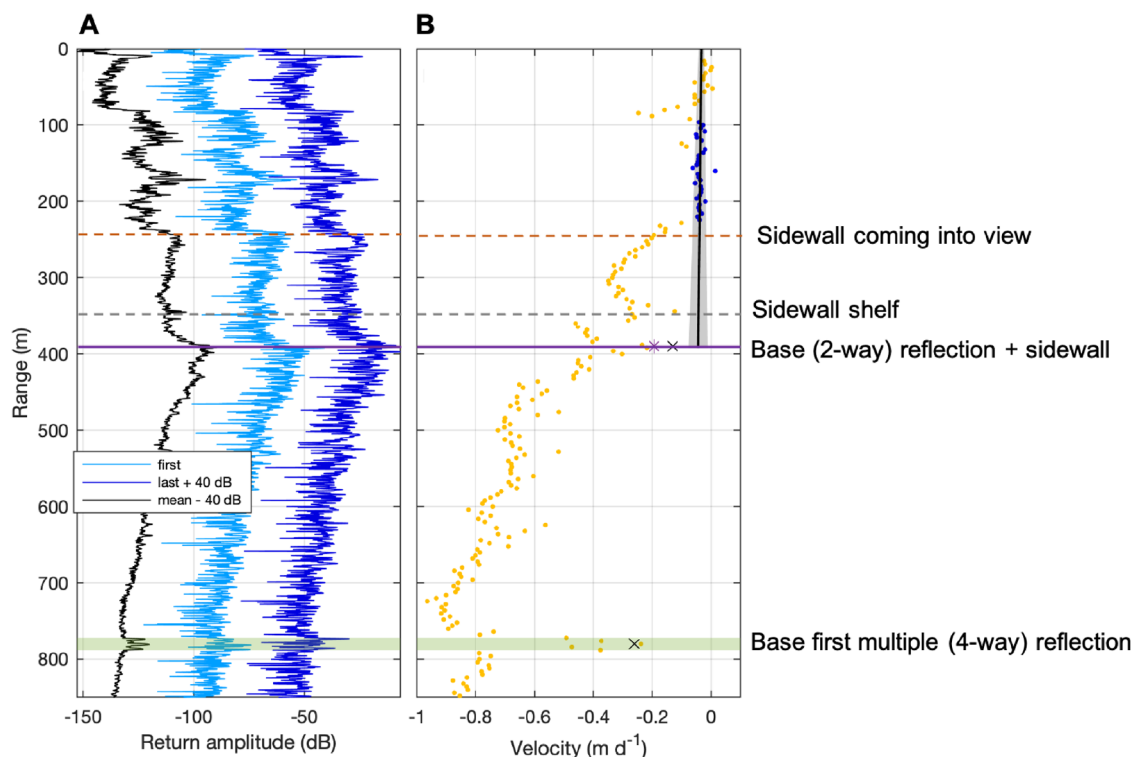
Figure 3. Iceberg SF0419 ApRES range profiles show the return amplitude of the first and last shots, the time-mean return (offset by 40 dB for visibility), and mean velocities of each range bin (b, yellow dots), with respect to the ApRES antennas at the iceberg surface (negative velocity is motion toward the antennas). Prominent features of the ApRES profiles are noted, including data used to calculate the vertical strain thinning rate and surface melt rate (blue dots), the basal reflector (purple line) and its multiple (green line), and the visibility of the side wall reflections (dashed orange line) and a prominent ledge (dashed gray line). The line style indicates if the noted feature was identified using a combination of ApRES and iceberg geometry (dashed) or identified solely from ApRES reflections (solid). The thickness of the solid lines represents the range bin thickness used for tracking the respective reflector. The total thinning rate, derived from the basal reflector multiple, (black x on both the base and base multiple ranges) and derived from the first basal reflector (purple star on only the base range) are noted.
