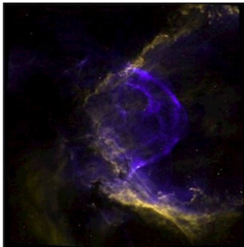
Figure 2. Change in the ionization state of the gas in NGC2359 illustrated as [\text{OIII}] in blue and [\text{OII}] in yellow.
