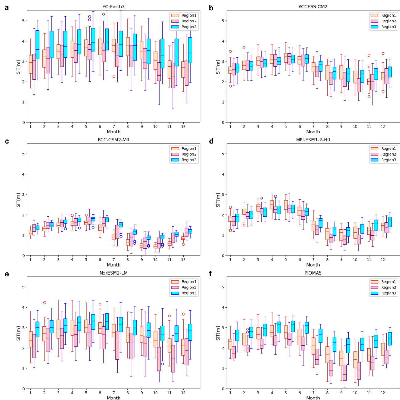
Figure 10. Regional comparison of monthly averaged SIT among region 1, region 2 and region 3 in the whole year, incorporating both five CMIP6 models (a) EC-Earth3, (b) ACCESS-CM2, (c) BCC-CSM2-MR, (d) MPI-ESM1-2-HR, and (e) NorESM2-LM and (f) PIOMAS data. Red boxes represent region 1, pink boxes represent region 2 and blue boxes represent region 3.
