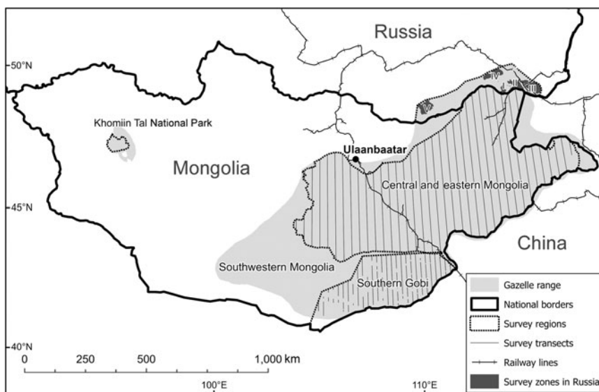
FIG. 1 Mongolian gazelle range and the population survey regions (central and eastern Mongolia, southern Gobi and Khomiin Tal National Park) during 2019–2020 in Mongolia. The 2020 gazelle population survey region in Russia comprises five zones (areas) including (I) Daursky Protected Area, (II) Dzeren Valley Protected Area, (III) west Krasnokamensk, (IV) north Onon River and (V) Sokhondinsky Nature Reserve and north Daursky.
