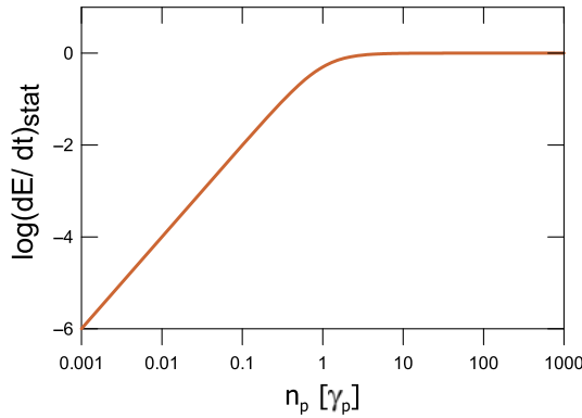
Figure 2. Power of the tidal energy dissipated in a planet in stationary rotation (arbitrary units) as a function of the orbital frequency (in units of \gamma_p ). In the case of gaseous bodies, n_p[\gamma_p] < 1 and, in the case of stiff planets, n_p[\gamma_p] > 1 .
