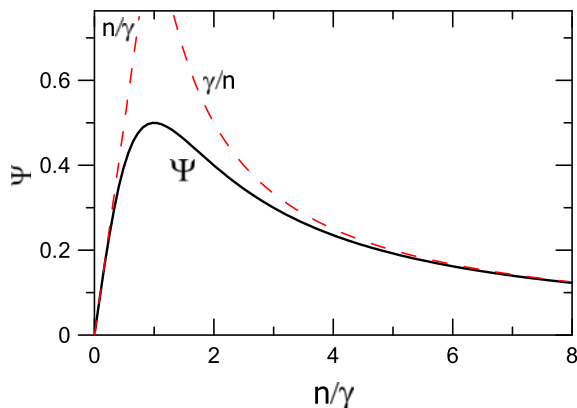
Figure 1. The function \Psi = (\gamma/n + n/\gamma)^{-1}
