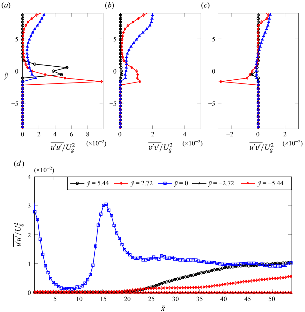
Figure 10. Profiles of (a) \overline{u'u'}/U_g^2 , (b) \overline{v'v'}/U_g^2 and (c) \overline{u'v'}/U_g^2 at different streamwise stations \tilde{x} : 0.55 (black circles), 21.76 (red diamonds), 53.31 (blue triangles). (d) Profiles of \overline{u'u'}/U_g^2 at different \tilde{y} stations. REF case of table 3.
