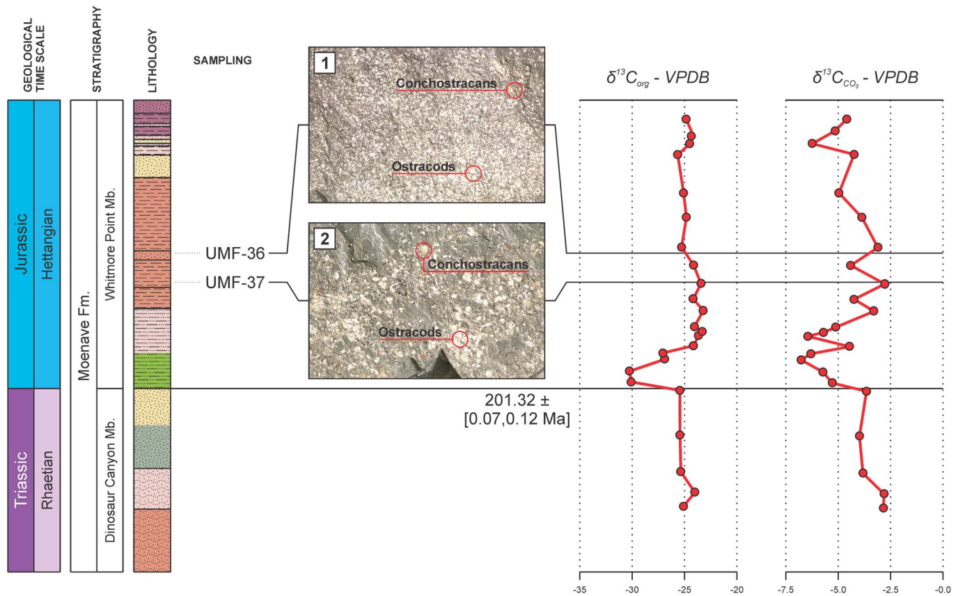
Figure 6. Ostracode extinction levels observed in the present work (1, 2) in comparison with the inorganic and organic carbon isotope curves ( \delta^{13}\text{C} ) of the Potter Canyon section (Suarez et al., 2017), Mohave County, Arizona, USA. Note the up-and-down trend of the inorganic ( \text{CO}_2 ) curve (VPDB = Vienna Pee Dee Belemnite standard).
