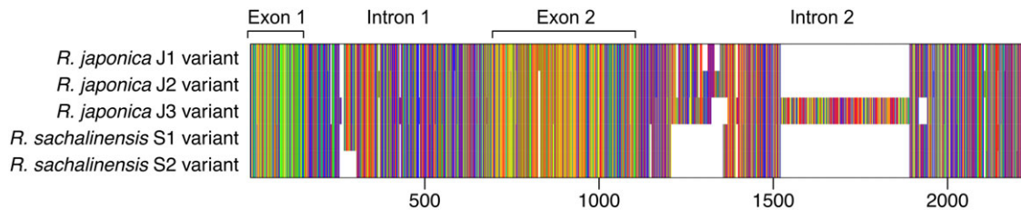
Figure 2. Alignment of LEAFY sequences for invasive Reynoutria taxa, showing the most commonly encountered sequences for each sequence variant. Sequences are identified as originating from R. japonica (J1/J2/J3) or R. sachalinensis (S1/S2). Intron and exon borders are indicated; the third exon is not shown but would appear shortly to the right of the last nucleotide shown.
