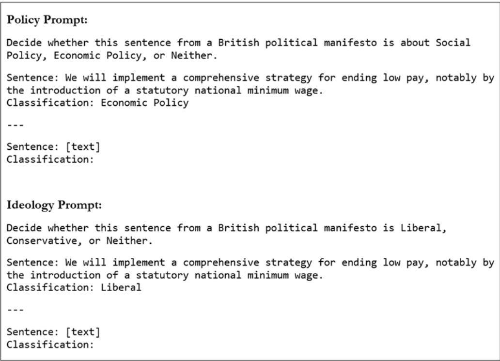
Figure 5. LLM prompt for ideology scaling task.
