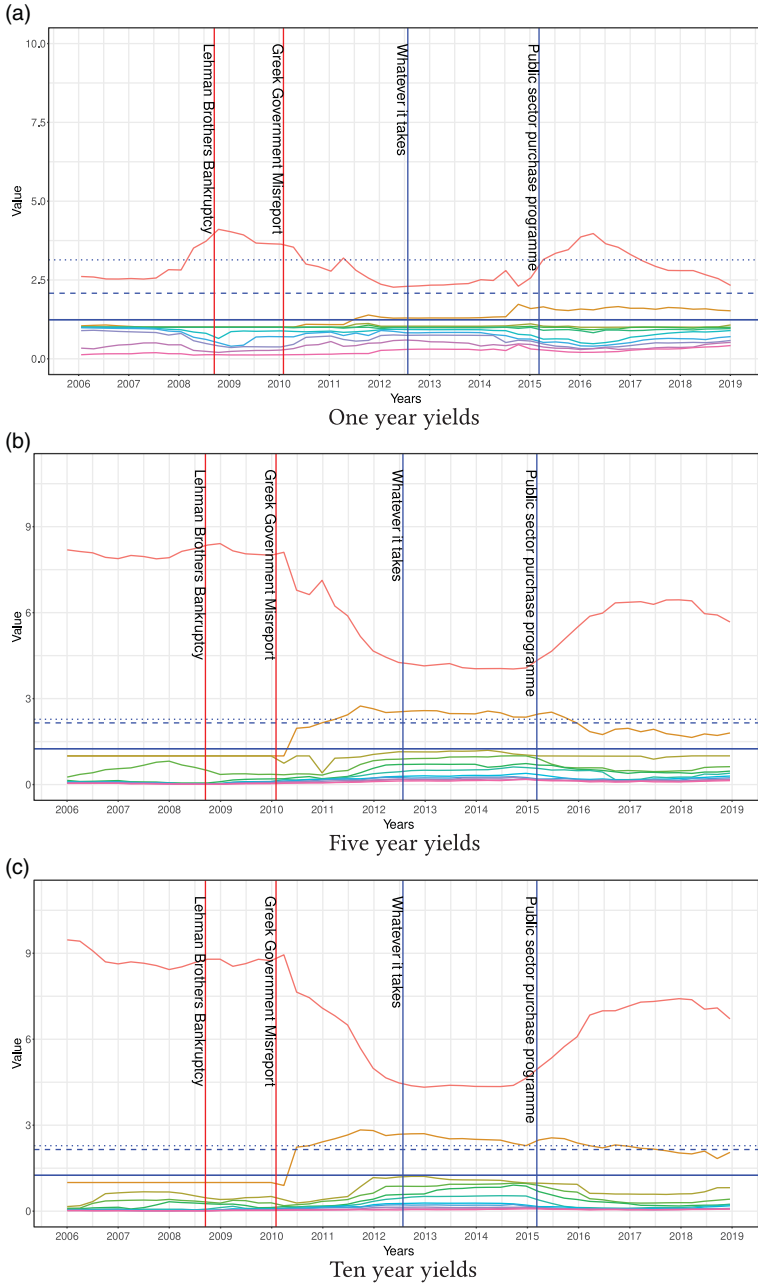
Figure C2. Eigenvalue evolution with optimal parameters for first difference. Notes: the full line indicates the Marčenko–Pastur theoretical bound, the dotted line indicates the simulated random model, and the thin dotted line indicates the rotational random model. For both the simulated random model and rotational random shuffling, 300 Monte Carlo simulations have been run. The dimension of the windows of the random matrix theory are reported in Table C1 in Section C.2 (in short, windows' width of 783 observations, i.e. 3 years, and step of 65 observations, i.e. one-quarter).
