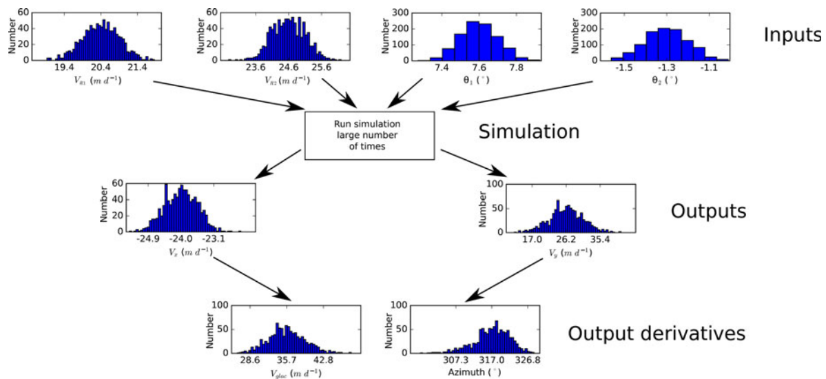
Fig. 5. A visual example of a Monte Carlo simulation (1000 runs) for a single point on the glacier surface. Here, the inputs are the radar velocity measurements ( V_{R1} and V_{R2} ) and their respective view directions ( \theta_1 and \theta_2 ). Note that we only obtain the distributions of V_x and V_y using the simulation. We then calculate the azimuth and velocity magnitude along with their respective uncertainties from the results of the simulation. This process is repeated for every desired data point over the glacier surface to produce Figures 6, 7.
