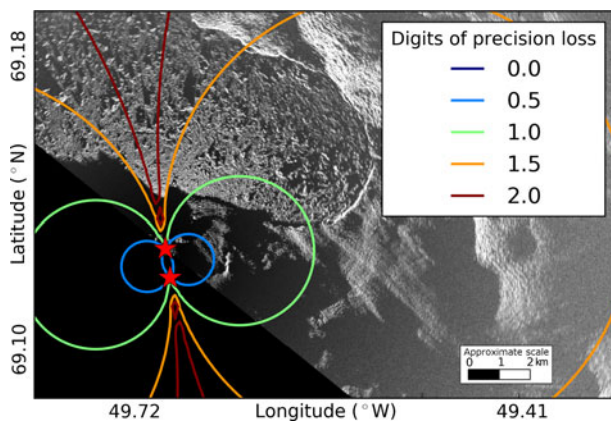
Fig. 9. Contours of loss of digits of precision considering the positions of the two radars (red stars) calculated from the condition number of the matrix of coefficients in Eqns (5) and (6). Most of the terminus experiences between 0.5 and 1.5 digits of loss.
