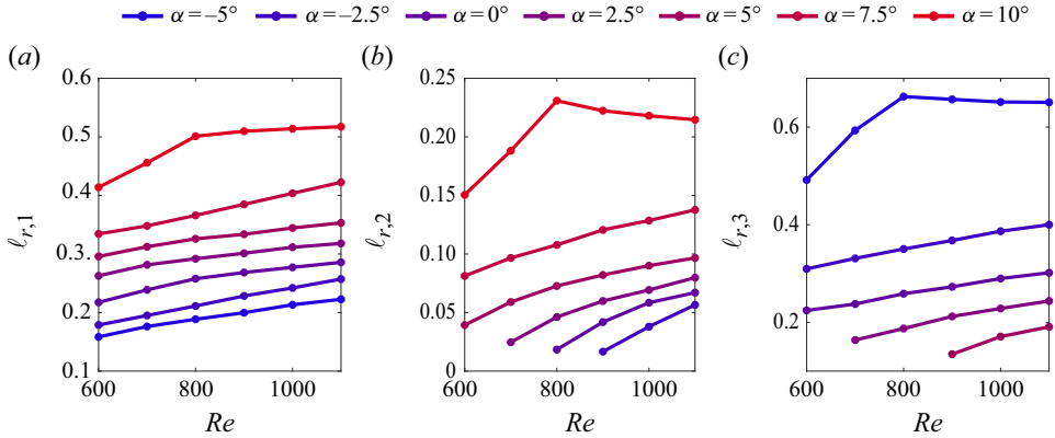
Figure 8. Dependence of the length of the main base flow recirculating regions on Re . See text for the definition of \ell_{r,1} , \ell_{r,2} and \ell_{r,3} . The size of the recirculating regions are measured using the delimiting \Psi = 0 line; when the \Psi = 0 line delimits two recirculating regions (see for example figure 7d), the position of the ensuing hyperbolic stagnation point is used as the delimiting point.
