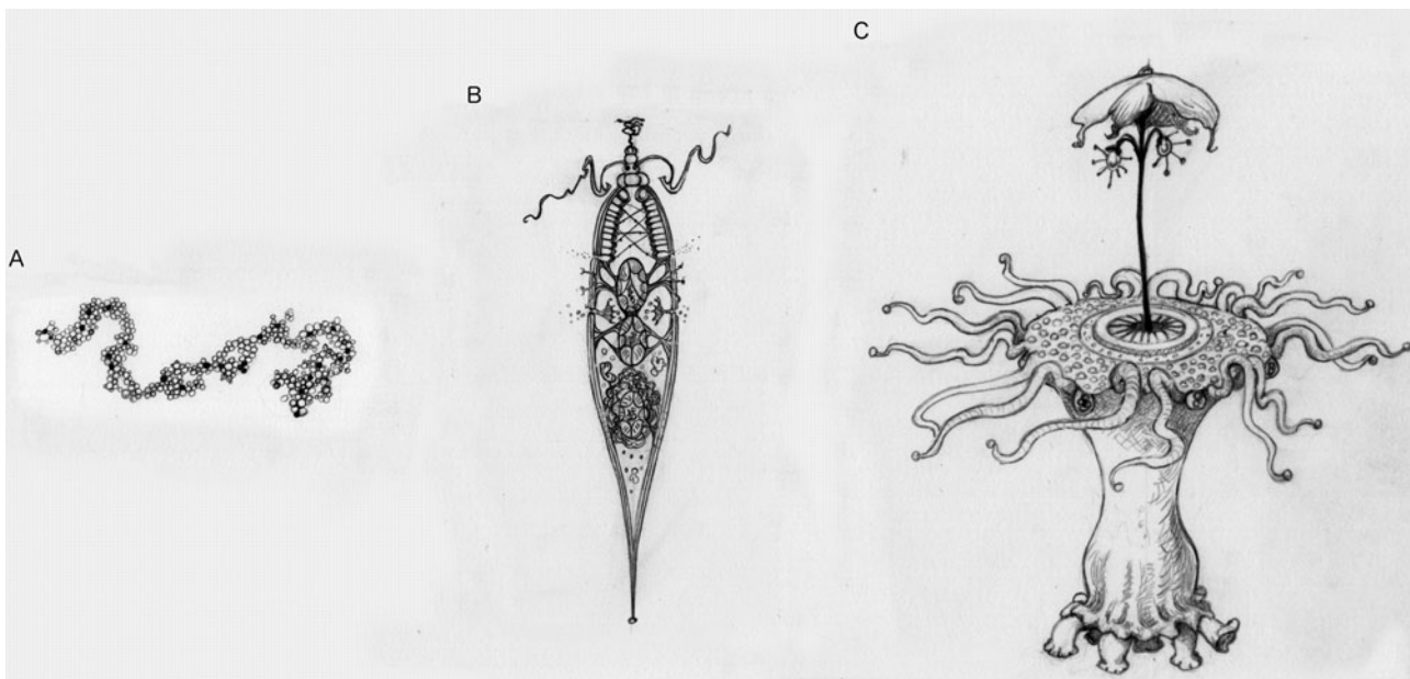
Fig. 2. Picture an alien. These illustrations represent different levels of adaptive complexity we might imagine when thinking about aliens. (a) A simple replicating molecule, with no apparent design. This may or may not undergo natural selection. (b) An incredibly simple, cell-like entity. Even something this simple has sufficient contrivance of parts that it must undergo natural selection. (c) An alien with many intricate parts working together is likely to have undergone major transitions.
