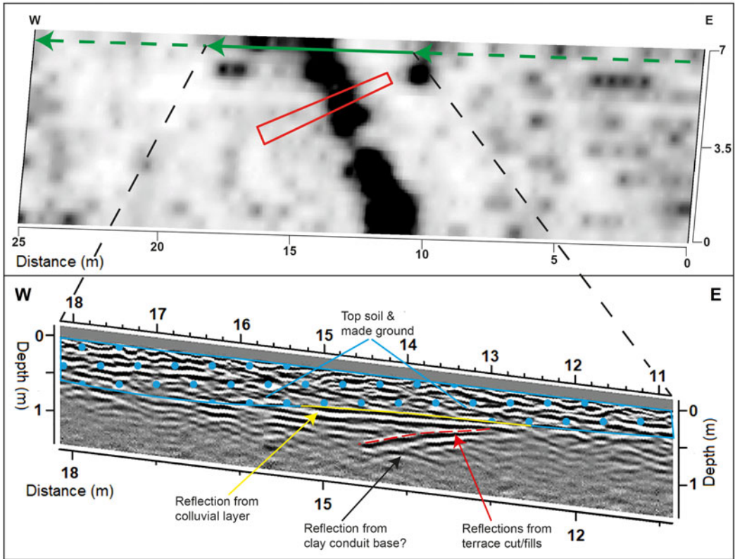
FIG. 5. Top: GPR amplitude time-slice showing the reflection of the line clay base of the aqueduct conduit, in relation to excavation Trench 1 (red outline). Bottom: A section of a topographically corrected GPR profile is interpreted as showing the hyperbolic reflection (indicated by the black arrow) caused by the clay base of the channel, the terrace (red dashed line), and the strong reflection from the fine colluvium layer formed after the aqueduct went out of use (yellow line – see the FIG. 7 section). Over this is a layer of made ground and colluvial subsoil (blue dots) lying under the current turf and topsoil. The location of this GPR profile is shown as the green line on the top illustration.
