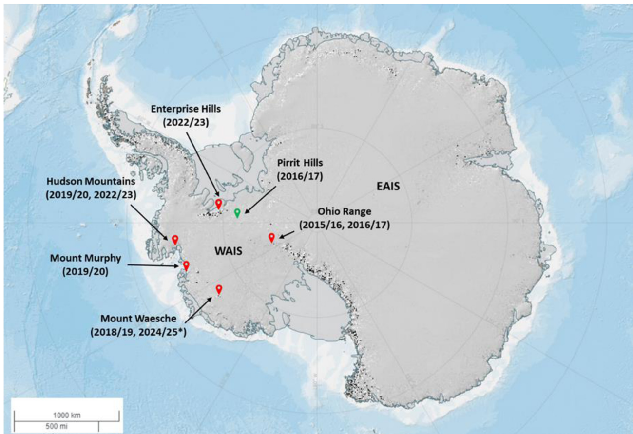
Figure 1. Overview map of Antarctica showing study locations and campaign dates of subglacial drill sites. Previously drilled sites include Ohio Range, Mt. Murphy (Kay Peak), Hudson Mountains (Winkie Nunatak), and Enterprise Hills. A reconnaissance geophysical survey was conducted at Mt. Waesche in 2018/19 with drilling proposed to begin in 2024/25 as noted by the asterisk. Red pins indicate Winkie Drill sites. The green pin indicates an additionally mentioned drill site that used the Agile Sub-Ice Geologic Drill (ASIG), capable of drilling to depths of 700 m. WAIS – West Antarctic Ice Sheet. EAIS – East Antarctic Ice Sheet. Textured gray represents the current ice-sheet surface (from Reference Elevation Model of Antarctica [Howat and others, 2019]). Shaded gray areas outlined in blue represent ice shelves. Bathymetry (blue and white shades) is from GEMCO2019 global dataset (GEMCO group, 2019). The basemap was created from the SCAR Antarctic Digital Database.
