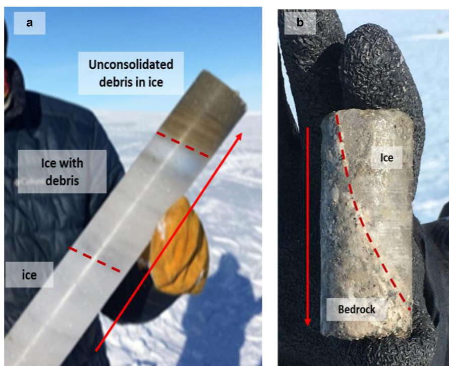
Figure 8. (a) A photo of a core collected from Mt. Murphy that illustrates increasing debris density downcore. These fine debris and clay material can delay or hamper drilling efforts for the Winkie Drill system. (b) Photo of a core collected from Ohio Range. The core was recovered with the basal ice frozen directly to the bedrock. The red arrow in each photograph is pointing downcore.
