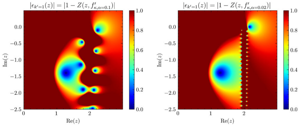
FIGURE 9. Root structures for the smooth cut-off distribution f_{\log,\alpha} with \alpha = 0.1 (left) and \alpha = 0.02 (right). The support function F_0 is a \kappa = 1 distribution with v_t = \sqrt{2} and the cut-off is at v_c = 2 .
