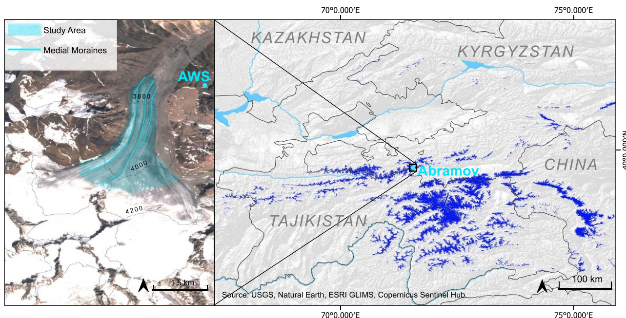
Figure 1. Right panel: Map showing the glaciated areas (dark blue) in Central Asia. Left panel: Overview of Abramov glacier, on a section of a Sentinel-2 scene (20 August 2019) overlaid with elevation data from Shuttle Radar Topography Mission (SRTM) imagery. The study area is outlined (light blue), using the Global Land Ice Measurements from Space (GLIMS) dataset, modified to reflect the 2020 glacier terminus as delineated by Enrico Mattea in Mattea and others (2024). The automatic weather station (AWS) location and the manually delineated supra-glacial medial moraines are also indicated.
