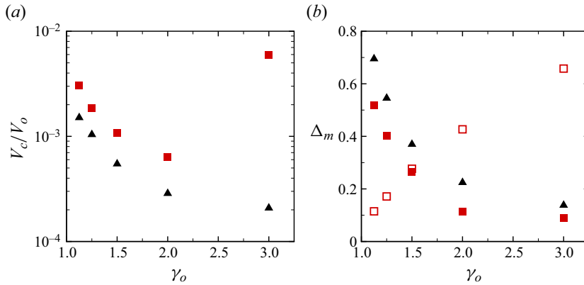
Figure 11. Bubble collapse volume vs stand-off distance (a) with no shear flow ( \omega_o = 0 ) ( \blacktriangle ) and shear flow ( \omega_o = 1/2 ) ( \blacksquare , red), and bubble centroid migration distance vs stand-off distance (b) with \Delta_z ( \blacktriangle ) for the case with no shear and \Delta_z ( \blacksquare , red) and \Delta_x ( \square , red) for the case with shear ( \omega_o = 1/2 ). Data with no mean shear flow were taken with permission from Rodriguez et al. (2022).
