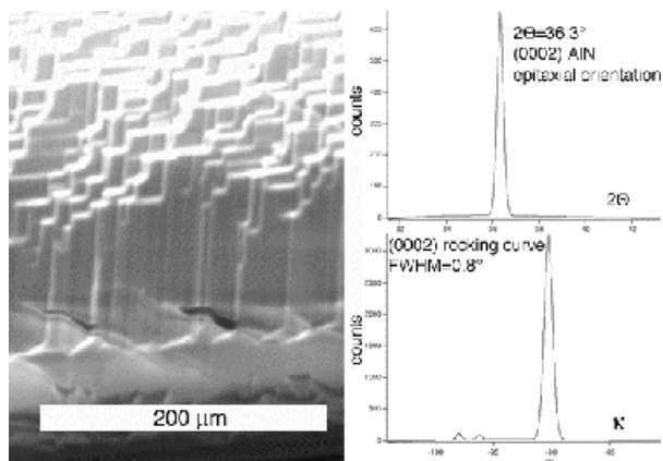
Figure 5. SEM image of a cleaved cross-section of an AlN crystal (left) and XRD analysis (right).
