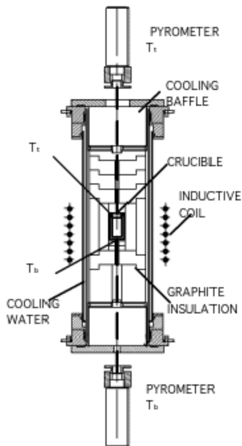
Figure 1. Schematic diagram of the inductively heated sublimation reactor. T_t and T_b refer to the top and bottom crucible temperatures, respectively.
