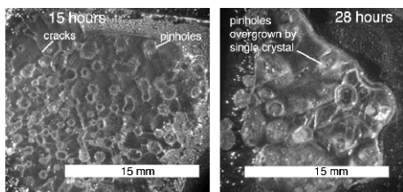
Figure 3. The effect of growth time on AlN crystal morphology at T_G=1930^\circ\text{C} and a source-to-seed distance of 10 mm. Left: AlN single crystal, 200-300 mm 2 large and 300-350 \mu\text{m} thick, after 15 hours of growth; Right: AlN single crystal, 200-300 mm 2 large and 650-700 \mu\text{m} thick, after 28 hours of growth.
