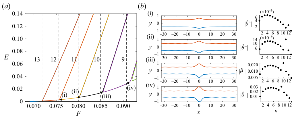
Figure 13. (a) Speed–energy bifurcation curves for R_1 = 1.01 , R_3 = 0.99 , h_1 = 50 , h_3 = 50 and k = 0.096 . The vertical dashed lines denote the predicted value of F where the mode-2 waves are resonant with the mode-1 waves having waves number nk . The corresponding values of n are shown close to the vertical lines. (b) Typical wave profiles and related absolute value of one of \hat{\theta}^\pm of the labelled solutions (i) to (iv) in (a), where \hat{\theta}^- and \hat{\theta}^+ are the Fourier coefficients of the inclination angle of the lower and upper interface.
