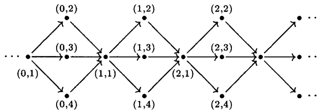
Figure 4. The quiver Z\Delta for \Delta of type D_4 . The vertices in \text{mod}A are labeled.
