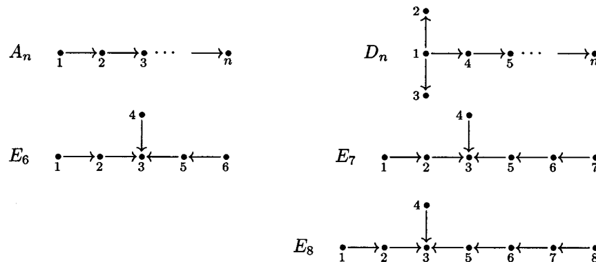
Figure 2. Orientations for the Dynkin graphs.
