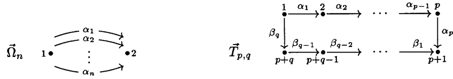
Figure 6. The quivers \Omega_n and T_{p,q} .
