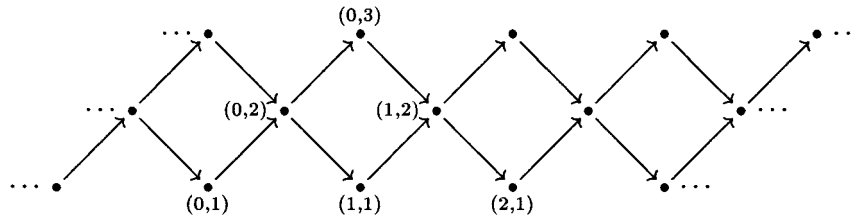
Figure 3. The quiver Z\Delta for \Delta of type A_3 . The vertices in \text{mod}A are labeled.
