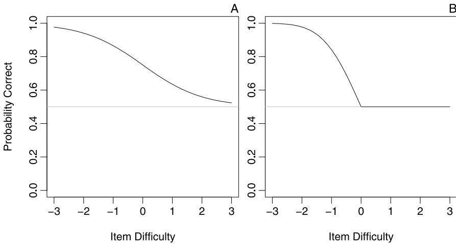
FIGURE 1. A. Person-response function for the average person in 1PL. B. The same for the 1P-MAC model.
