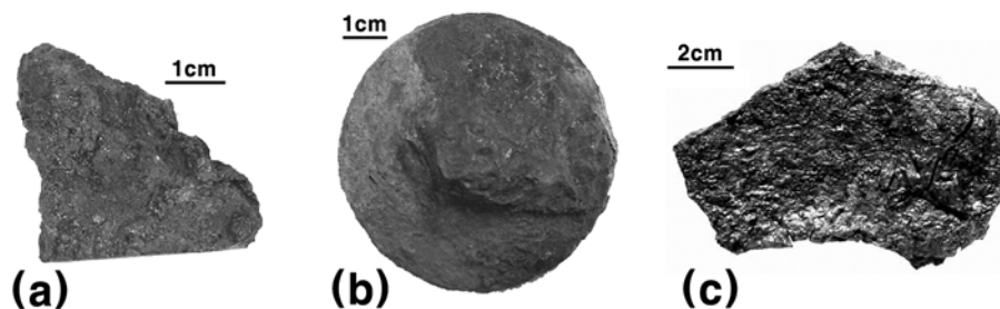
Figure 2 General appearance of cast iron objects examined: (a) piece from a Koguryo site at 1 in Figure 3; (b) a circular button from a Paekche site at 2 in Figure 3; (c) fragment of a cauldron from a Silla site at 3 in Figure 3.
