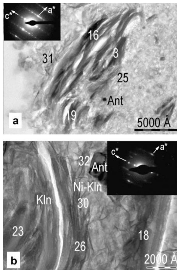
Figure 3. (a) Low-magnification TEM image of a typical kaolinite stack from sample XM-30, enclosed within a fine-grained matrix of Ni-rich particles. (b) Curved particles of Ni-rich kaolinite form the external zones of the stack and also appear as isolated curved particles. The SAED pattern of the stack (inset) reveals the presence of kaolinite particles with variable orientation and sharing the c^* axis. The numbers correspond to the analyses reported in Table 4. Kln: kaolinite; Ant: anatase.
