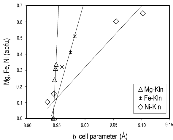
Figure 9. Plot of Mg, Fe and Ni contents (a.p.f.u.) vs. the b cell parameter in Mg-kaolinite (Bentabol et al. , 2006), Fe-kaolinite (Iriarte et al. , 2005) and Ni-kaolinite (this study).
