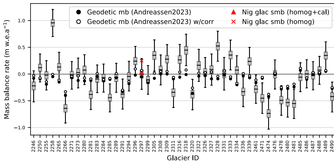
Figure 9. Modelled glacier-wide SMB rate over mass-balance years 1967–2020 for 48 glaciers of Jostedalbreen (boxplots) with geodetic mass-balance estimates for 1966–2020 (points; Andreassen and others (2023)). Black horizontal lines in boxplots show medians, grey shaded areas show IQR (Q1–Q3) and whiskers extend to 1.5 IQR. Black points show uncorrected geodetic mass balance, while white points show geodetic mass balance corrected for internal ablation and additional melt from mapping dates to end of melt seasons (Andreassen and others, 2023). Glaciological glacier-wide SMB rate for Nigardsbreen over the same period shown as triangle (homogenized and calibrated record) and cross (homogenized only). Detached tongue of Brenndalsbreen (ID2301) not included due to scale (very negative median modelled SMB rate -3.70 m w.e. a^{-1} with poor correspondence to geodetic rate -0.54 m w.e. a^{-1} ).
