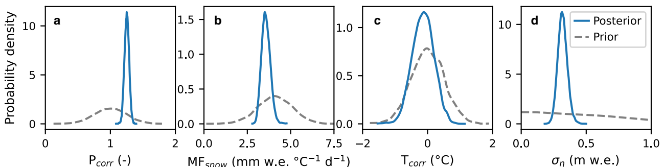
Figure 2. Marginal prior (grey dashed lines) and posterior (blue solid lines) probability distributions of global parameter set: (a) precipitation correction factor P_{\text{corr,glob}} , (b) melt factor for snow MF_{\text{snow,glob}} , and (c) temperature bias correction T_{\text{corr,glob}} and (d) SD in model error \sigma_\eta .
