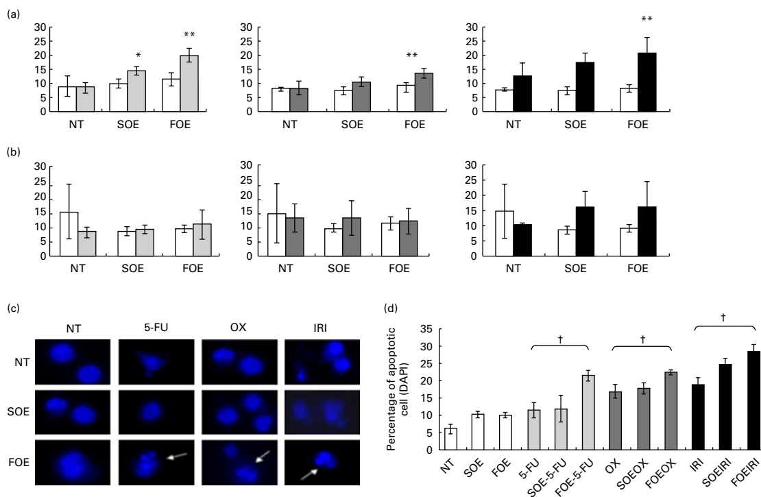
Fig. 2. Apoptosis induction was evaluated after a 24-h treatment with 1 \mu\text{M} -5-fluorouracil (5-FU, \square ), 1 \mu\text{M} -oxaliplatin (OX, \blacksquare ) or 10 \mu\text{M} -irinotecan (IRI, \square ) in combination or not with fish oil emulsion (FOE) or soyabean oil emulsion (SOE) in (a) HT-29 and (b) LS174T cells, using fluorescence-activated cell sorter analysis with annexin-V-fluorescein isothiocyanate and propidium iodide staining. Values are means and standard deviations for three independent experiments (** P < 0.05 FOE/chemoT v. chemoT, * P < 0.05 SOE/chemoT v. chemoT). The percentage of HT-29 apoptotic cells was also evaluated through nuclear morphological changes, using 4',6'-diamidino-2-phenylindole staining. (c) White arrows indicate nuclei condensation and apoptotic body formation. (d) Statistical analysis showed a significant difference between samples with or without FOE in the context of 5-FU, OX or IRI treatment †( P < 0.05 ). NT, Not treated. (A colour version of this figure can be found online at http://www.journals.cambridge.org/bjn )
