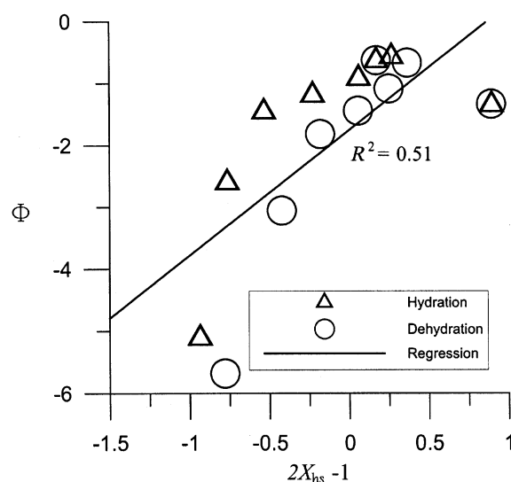
Figure 9. Using the linear relationship of \Phi vs. ( 2X_{\text{hs}} - 1 ) to obtain the slope -W_s/2.30RT and intercept ( \log K ).
