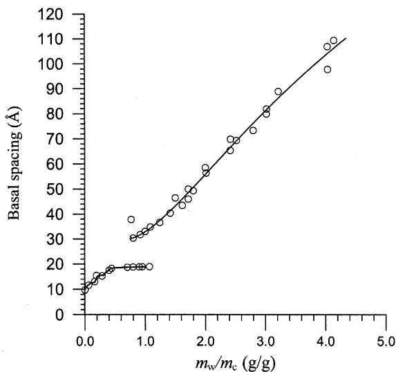
Figure 2. Basal spacing vs. the ratio of water mass ( m_w ) to smectite mass ( m_c ) in a Na-smectite water system (after Zhang and Low, 1989).
