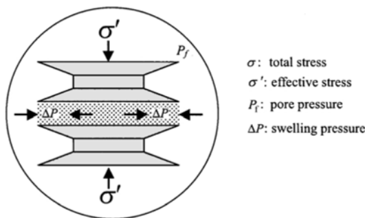
Figure 11. Schematic diagram of the equilibrium between swelling pressure and effective stress in the interlayer of Na-smectite (after Fitts and Brown, 1999).
