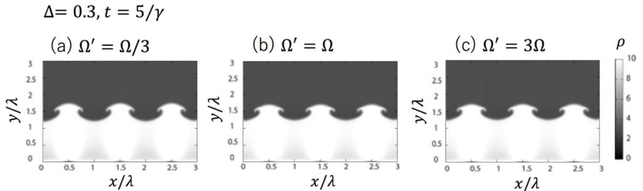
Figure 6. Fluid simulation results for the RTI mitigation for the time-dependent wobbling frequency \Omega(t) = \Omega(1 + \Delta \sin \Omega' t) at t = 5/\gamma . In the simulations \Delta = 0.3 , and (a) \Omega' = \Omega/3 , (b) \Omega' = \Omega and (c) \Omega' = 3\Omega . The dynamic mitigation mechanism is also robust against the time change of the perturbation frequency \Omega(t) .
