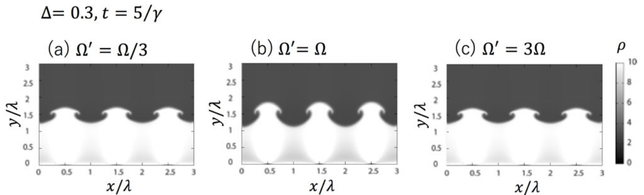
Figure 5. Fluid simulation results for the RTI mitigation for the time-dependent \delta g(t) = \delta g - \Delta \sin \Omega' t at t = 5/\gamma . In the simulations \Delta = 0.3 , and (a) \Omega' = \Omega/3 , (b) \Omega' = \Omega and (c) \Omega' = 3\Omega . The dynamic mitigation mechanism is robust against the time change of the perturbation amplitude \delta g(t) .
