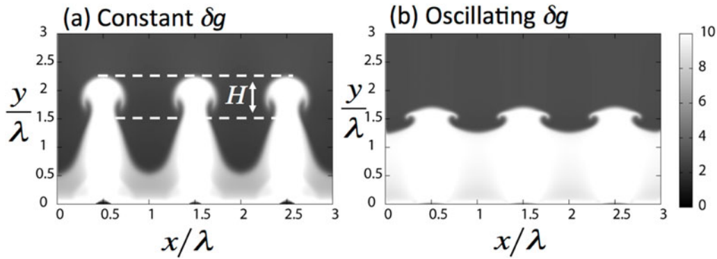
Figure 4. Example simulation results for the Rayleigh–Taylor instability (RTI) mitigation. \delta g is 10% of the acceleration g_0 and oscillates with the frequency of \Omega = \gamma . As shown above and in Equation (3), the dynamic instability mitigation mechanism works well to mitigate the instability growth.
