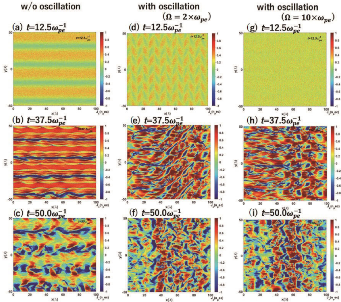
Figure 10. Filamentation instability simulation results without and with the electron beam oscillation. The current density J_x is shown at each time step. When the electron beam axis oscillates in the y direction ((d)–(f) and (g)–(i)), the filamentation instability growth is clearly mitigated.
