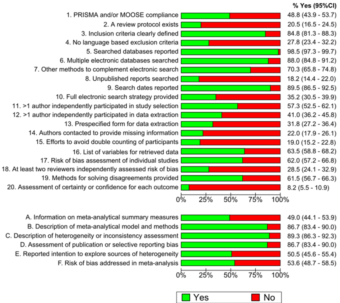
Figure 2. Distribution of fulfilled ReMarQ items (% Yes) of all systematic reviews (A) and of meta-analyses (B) Includes 400 systematic reviews stratified by JCR category (n = 38), where each category contributes with a similar number of systematic reviews (main analysis).
