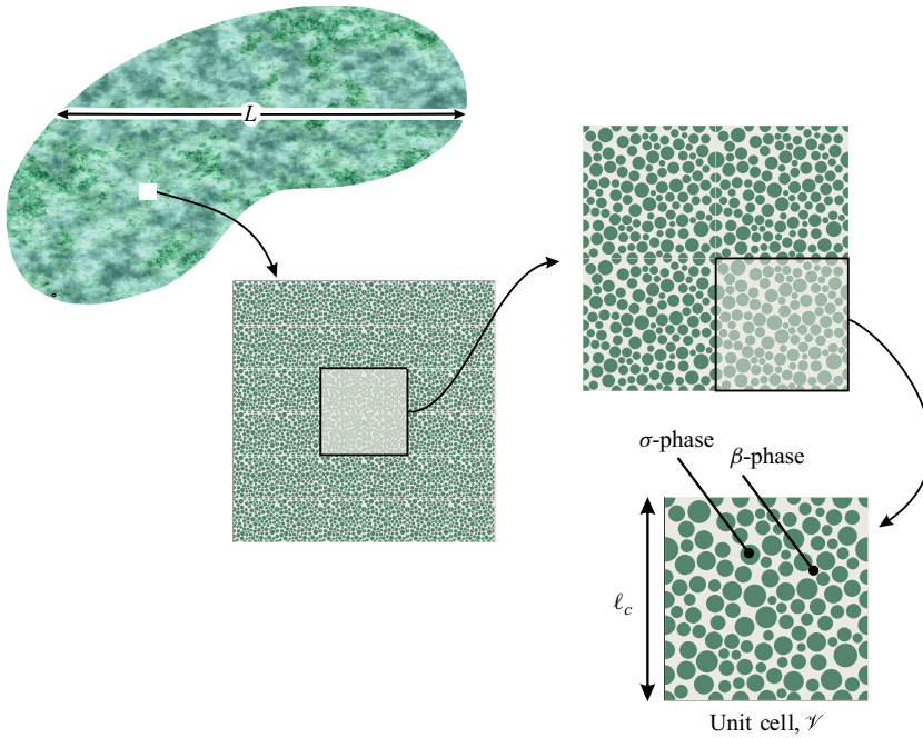
Figure 1. Sketch of a porous medium of characteristic length L that is represented as an array of periodic unit cells \mathcal{V} containing a fluid phase (the \beta -phase with characteristic length \ell_\beta ) and a solid phase (the \sigma -phase with characteristic length \ell_\sigma ).
