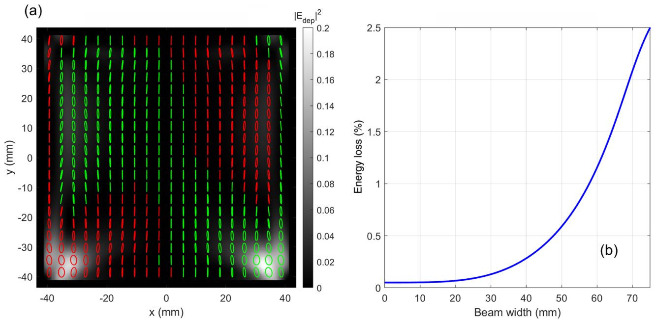
Figure 4. Simulation results for depolarization loss at 1060 nm with a quartz rotator placed between the two amplifiers and cut at a thickness to rotate the central wavelength's polarization by 90°.
