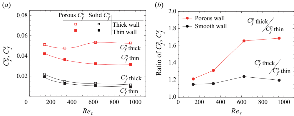
Figure 3. Skin friction coefficients at the porous/fluid interface ( C_f^p ) and at the smooth wall ( C_f^s ) against Re_\tau : (a) C_f^p and C_f^s for the thick- and thin-wall cases, and (b) the ratios of C_f^p and C_f^s for the thick-wall cases divided by the corresponding values for the thin-wall cases.
