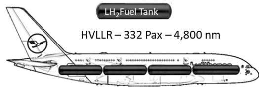
Figure 2. HVLLR airliner. Image courtesy [21], modified by the authors [13].
